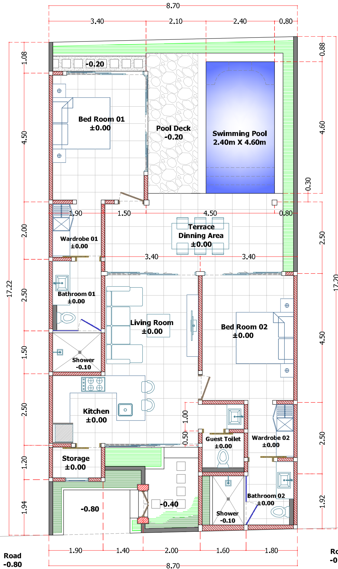
P L A N skala 1: 80
